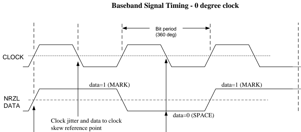
Figure 11: NRZ-L Signal Timing
