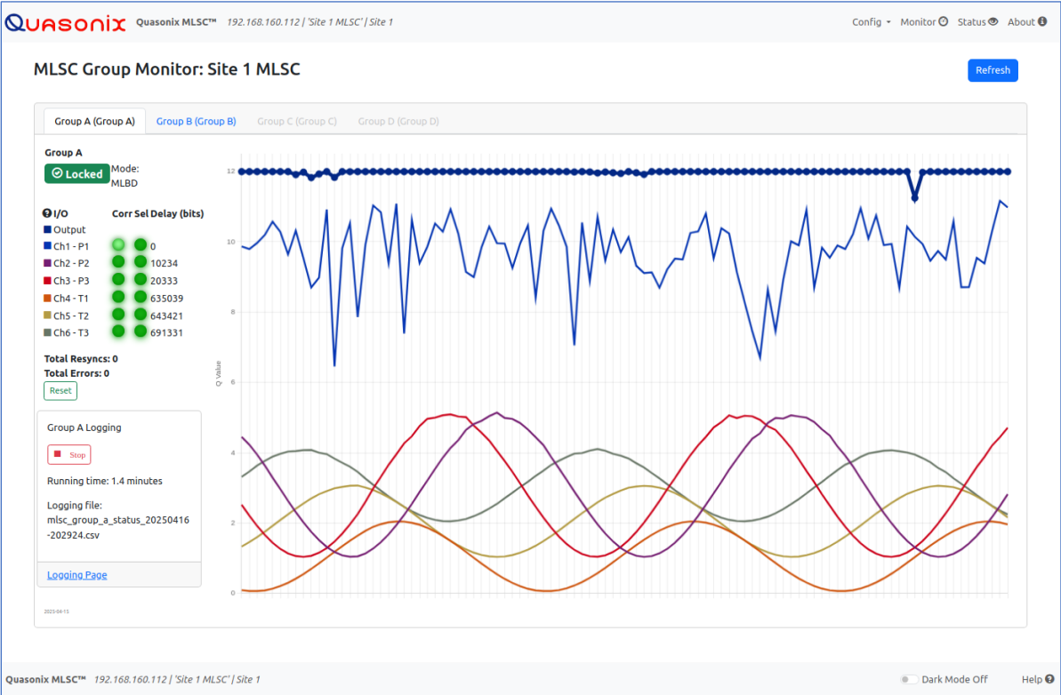
Figure 50: MLSC™ Group Monitor
