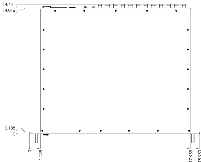
Figure 4: Mechanical Drawing – 1U Top View
