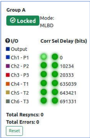
Figure 51: Text-Based Group Monitor Information
