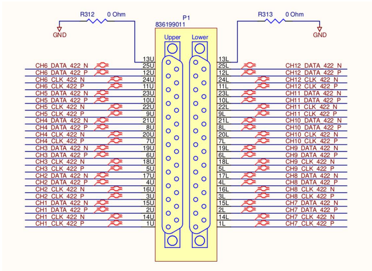
Figure 7: MDM-25 D-Sub Pin Locations for Ch 1-6 and Ch 7-12
