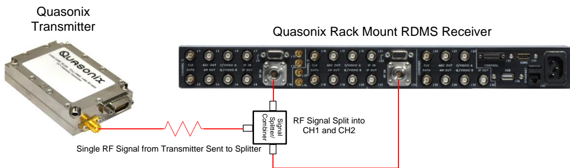
Figure 51: Example Bench RF Configuration for Single Transmitter and Rack Mount Receiver
