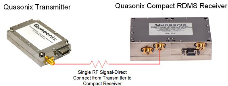
Figure 49: Example Bench RF Configuration for Single Transmitter and Compact Receiver
