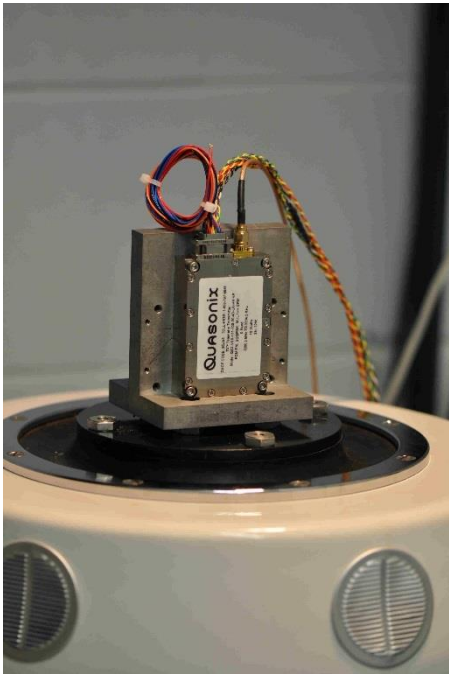
Figure 36: TIMTER™ Mounted for Y-axis Testing
