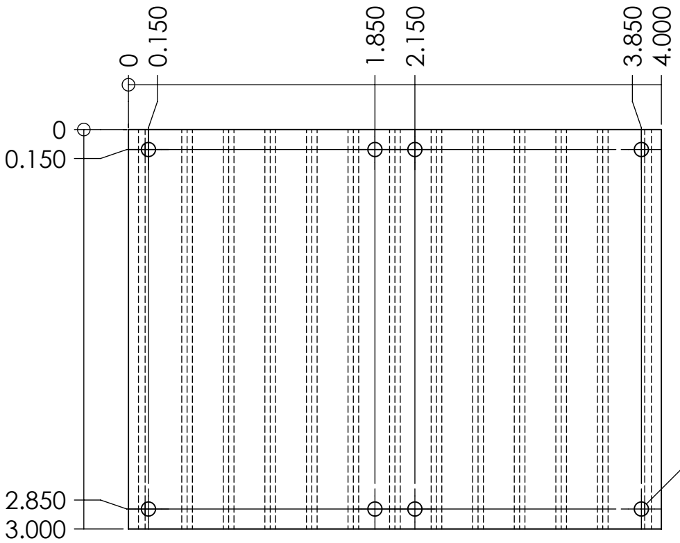
BOTTOM VIEW
